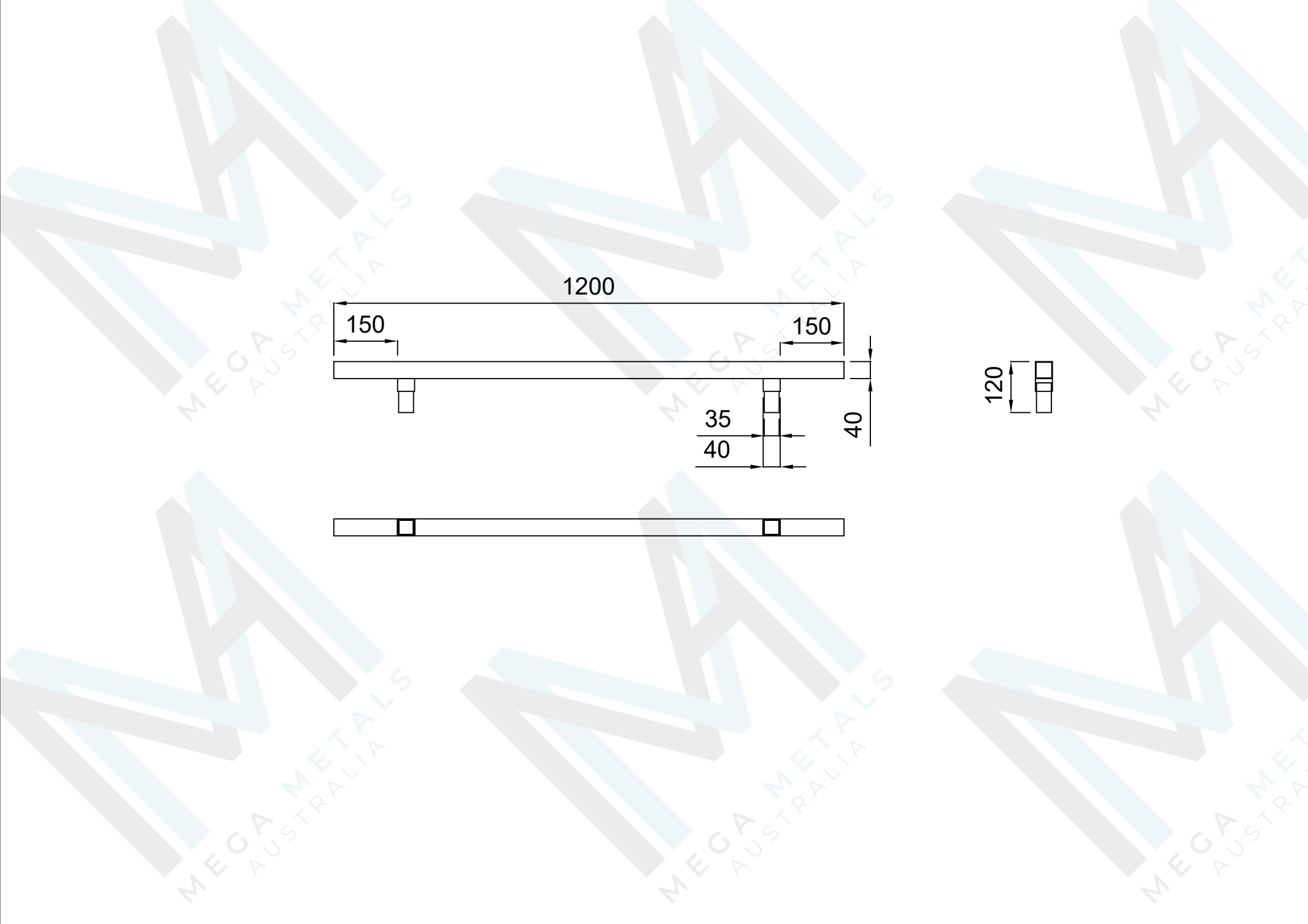
01 FRONT VIEW TO SCALE
