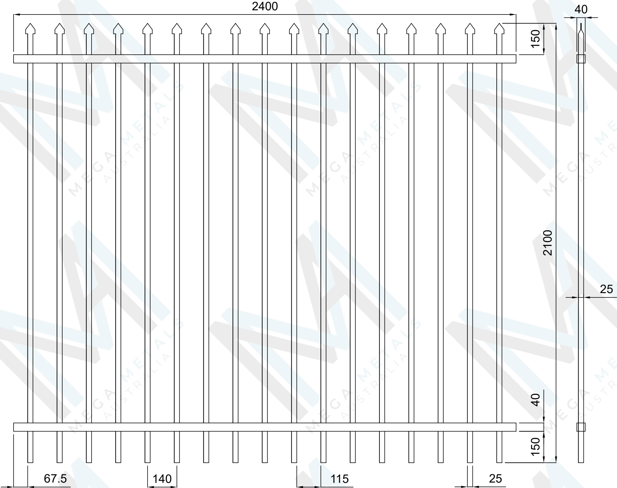
01 FRONT VIEW TO SCALE
