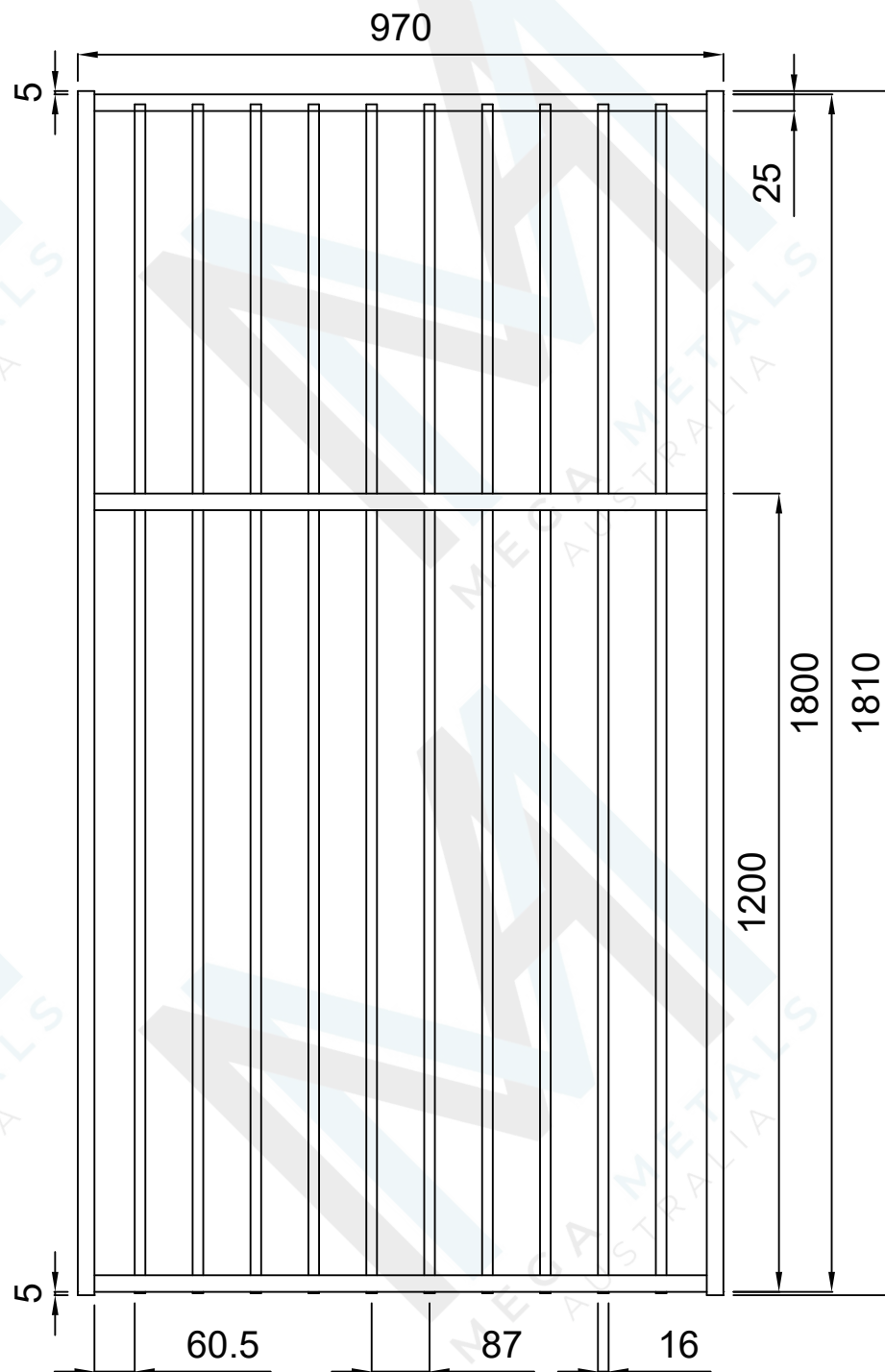
01 FRONT VIEW TO SCALE
