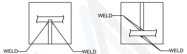
BOTTOM RAIL FRONT VIEW
