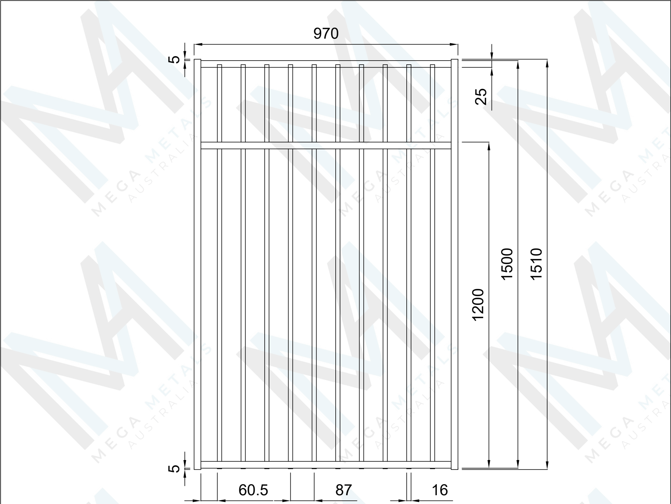
01 FRONT VIEW TO SCALE
