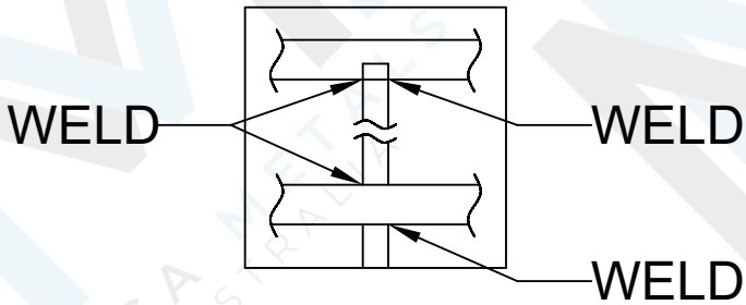
BOTTOM RAIL FRONT VIEW
